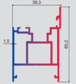
T.2157 1,002 kg/mt Kollu Profili
